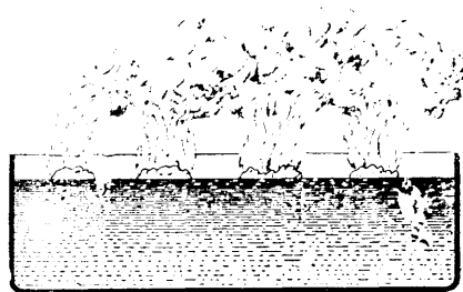
Fig. 7. Flame of solidified gas.
