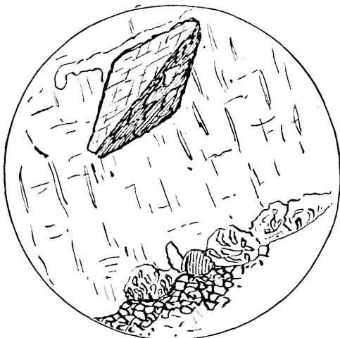
Fig. 8. Microcline containing Hornblende, Micropegmatite on e. ge. Redgut bay.
