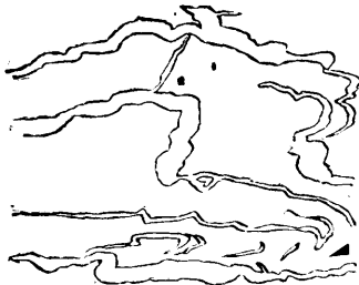
Fig. 5. Arrangements of veins in contorted schists.
