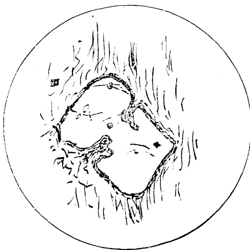
Fig. 11. Quartz Porphyrite. Rocky Narrows.
