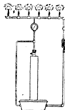
Fig. 10. Flame of liquefied acetylene.
