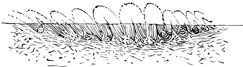
Fig. 1. Folds in Couchiching—after W. H. C. Smith, p. 55 G, Geol. Sur. Can., vol. V., Part I.
