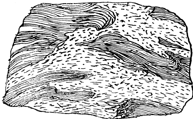
Fig. 7. Contact of Granitoid Gneiss and Couchiching. Goose Island, Rainy lake.
