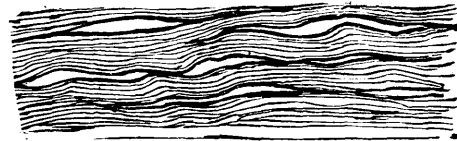
Fig. 4. Overlapping arrangements of bedded veins.
