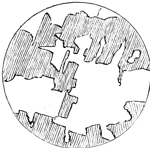
Fig. 15. Plagioclase, shaded in direction of striations, quartz white, lower part a single individual. Little Canada island.
