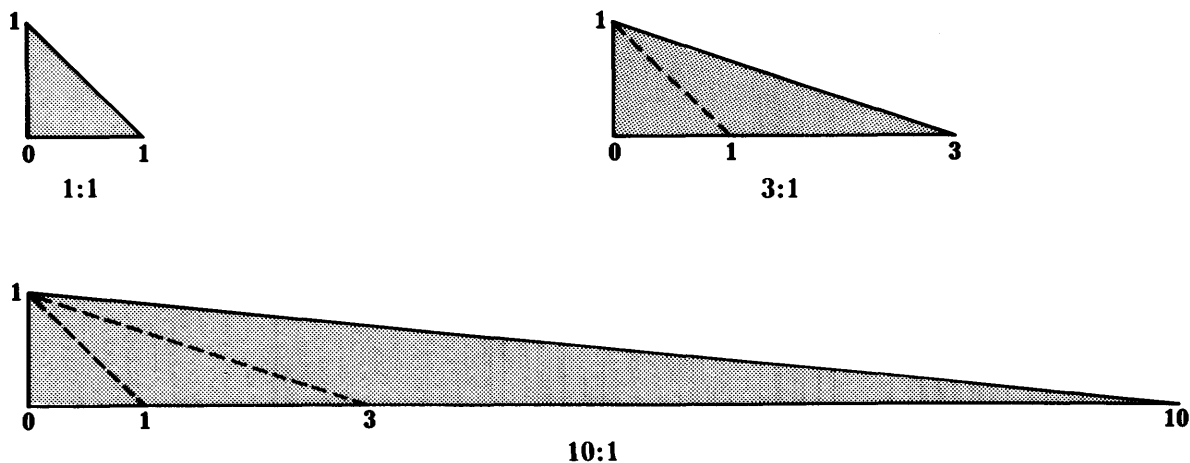
Figure 19. Slope gradients.
