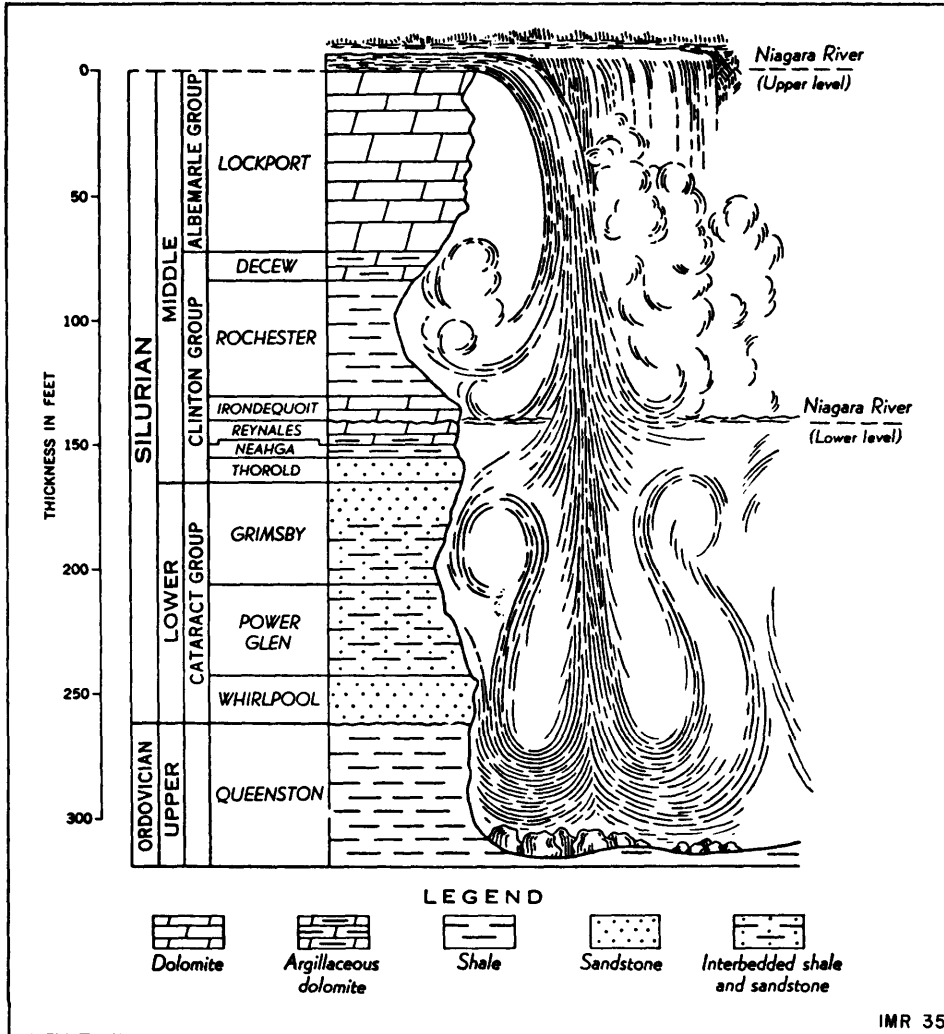
Figure 1 - Stratigraphic Section at Niagara Falls (courtesy of Geol. Surv. Canada)
