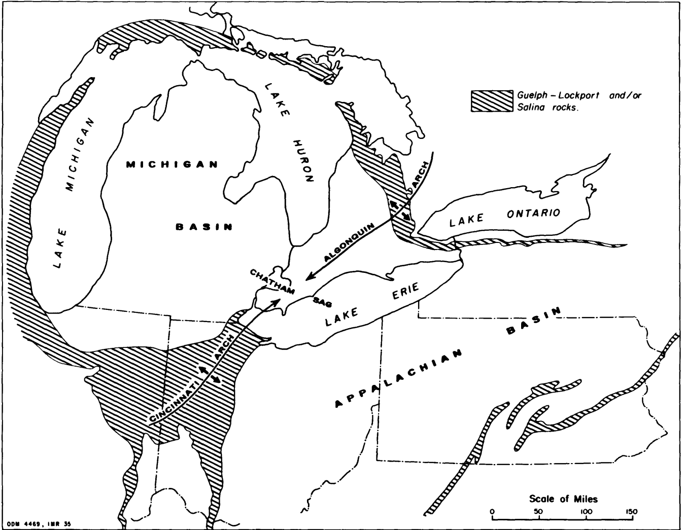
Figure 3 - Niagara Escarpment and major structural elements (from Vos 1969)
