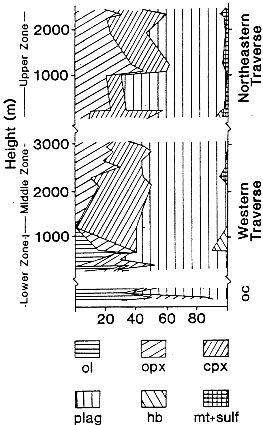
Figure 13. Petrographic traverse for cumulate rocks. ol -olivine; opx -orthopyroxene; cpx -clinopyroxene; plag -plagioclase; hb -hornblende; mt + sulf -magnetite and sulfide; oc - olivine-rich cumulates. Traverse locations shown in Figure 12.
