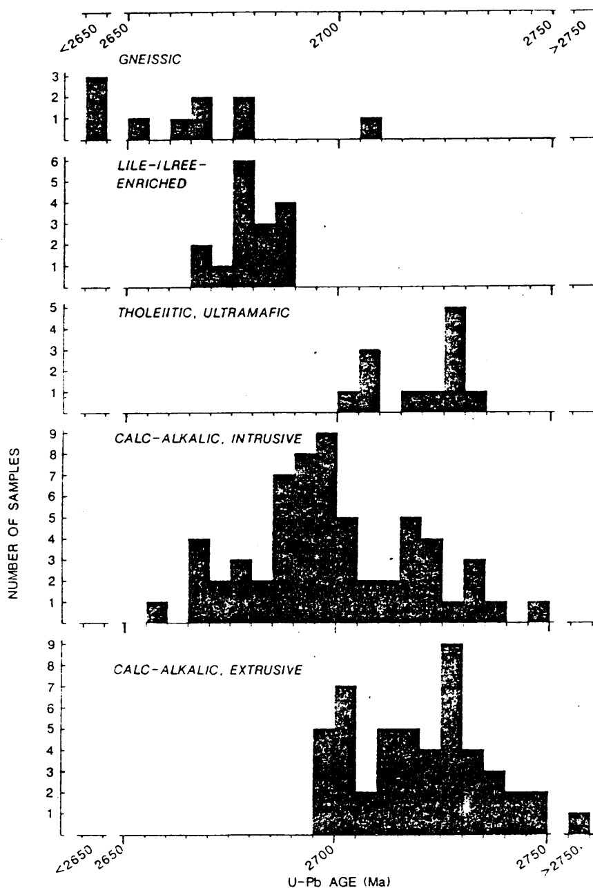
Figure 35. Histogram of high precision, U-Pb ages for the southern Superior Province (excluding well-defined basement terrane >2780 Ma, and samples with complex U-Pb data that do not clearly define primary igneous ages). The majority of these ages have 2-sigma errors of \pm 2 to 4 Ma. The ^{207}\text{Pb}/^{206}\text{Pb} ages for the detrital sedimentary grains generally have significantly larger errors: see references for details. Gneissic: predominantly calc-alkalic intrusive rocks at amphibolite or granulite facies in the Kapuskasing (or related) terrane; LILE-/LREE-enriched: intrusive and extrusive rocks, including one alkalic metavolcanic rock, an albitite dike, lamprophyres, and monzodiorite-syenite-granodiorite intrusions with alkalic affinity (e.g., Otto stock, Kirkland Lake area); Tholeiitic, Ultramafic: supracrustal tholeiitic intrusions and related metavolcanic rocks, and one ultramafic dike; Calc-alkalic, Intrusive: tonalite-trondjemite and diorite-granodiorite-granite intrusions, quartz-feldspar porphyries associated with gold mineralization, and sedimentary conglomerate clasts of these compositions; Calc-alkalic, Extrusive: rhyolites and dacites; Sedimentary Detrital:
