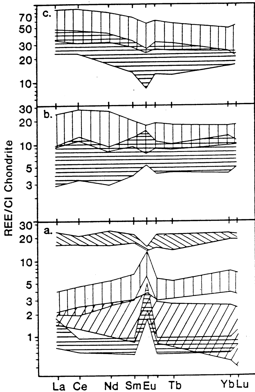
Figure 17. Rare earth element profiles, normalized to CI chondrite values of Evensen et al. (1978). Gd values determined from interpolation between Sm and Tb.
