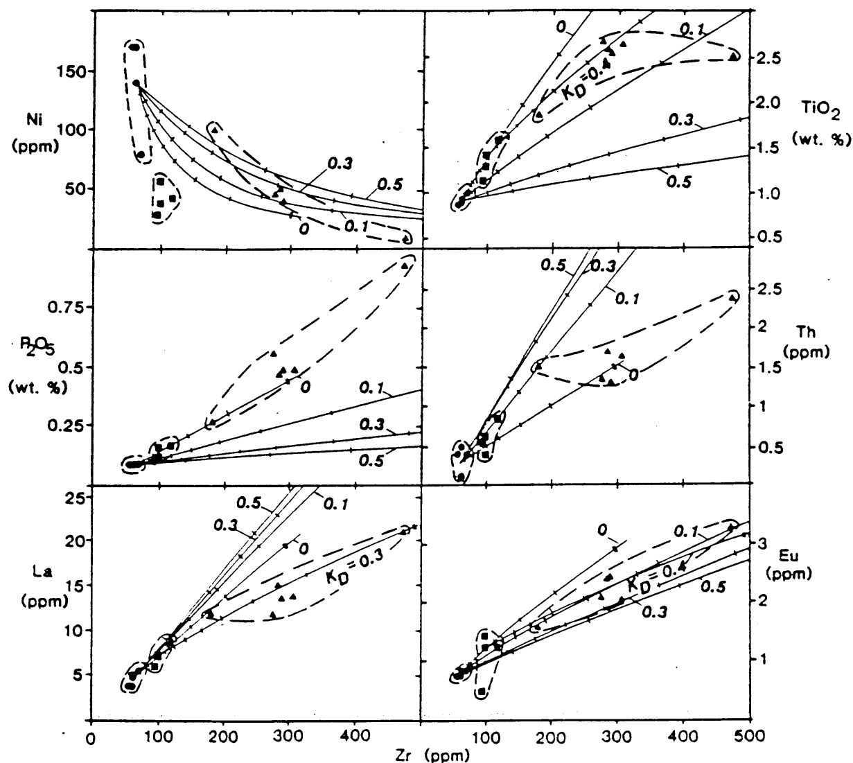
Figure 24. X-Y plots for liquid compositions with AFC modeling curves. KGC chill samples: dots; Kamiskotia "primitive" basalts: squares; Kamiskotia evolved basalts: triangles. AFC curves using equations of DePaolo (1981) labeled by ratio of mass assimilated (MA) to mass fractionated (MF), with 0 representing fractionation only. Tick marks represent 10% fractionation increments; double-tick marks are for 80% fractionation. Assimilant used is average of 9 granites and tonalites from the KGC granophyre, with 6 ppm Ni, 0.29 wt.% \text{TiO}_2 , 0.04 wt.% \text{P}_2\text{O}_5 , 9.2 ppm Th, 58 ppm La, 2.9 ppm Eu and 643 ppm Zr (Hart, 1984). Bulk K_D s used: Ni: 2; \text{TiO}_2 : 0.2; \text{P}_2\text{O}_5 : 0.01; Th: 0.001; La: 0.1; Eu: 0.2; Zr: 0.01. For \text{TiO}_2 , La and Eu, secondary FC curves from 100 ppm Zr use bulk K_D s as labeled. Additional data from Hart (1984) and Appendix V. a. Ni versus Zr. b. \text{TiO}_2 versus Zr. c. \text{P}_2\text{O}_5 versus Zr. d. Th versus Zr. e. La versus Zr. f. Eu versus Zr.
