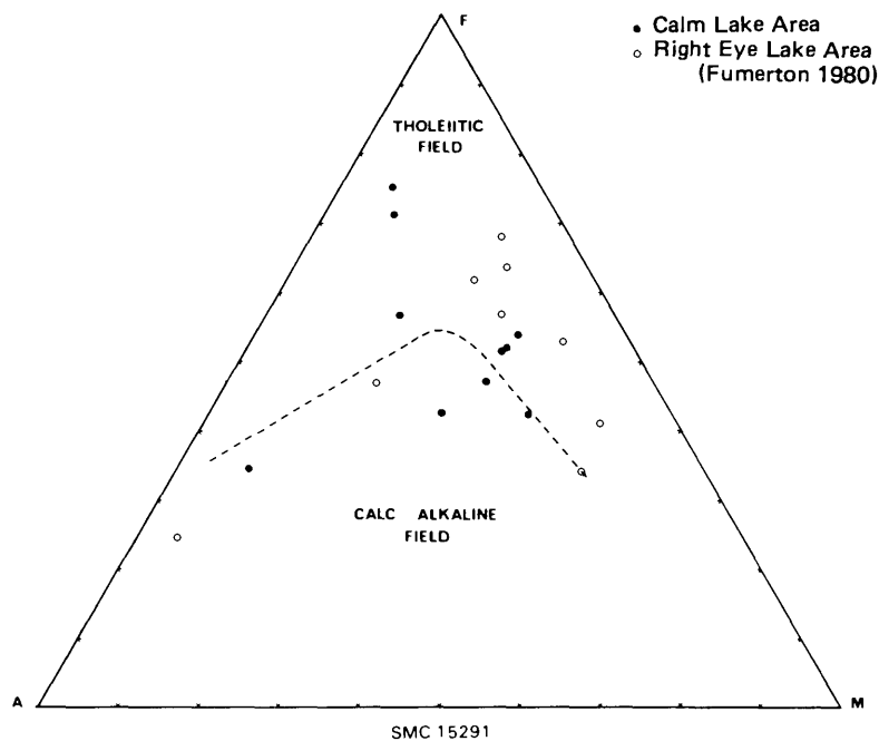
Figure 4. AFM plot for metavolcanics. The mafic flows are tholeiitic, pyroclastic rocks are calc-alkaline. Samples from Right Eye Lake area (Fumerton 1980) shown for comparison. Dividing line between tholeiitic and calc-alkaline affinities after Irvine and Baragar (1971).
