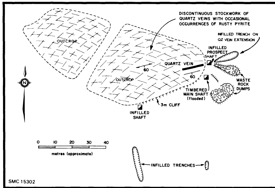
Figure 14. Sketch map of the geology of main workings at the Independence mine. Geology by S.L. Fumerton.
