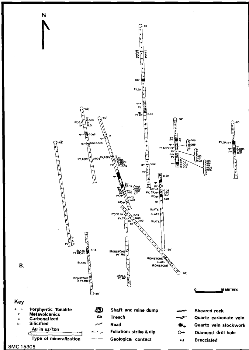
Figure 16b. Plan of diamond drill intersections, projected vertically, at the Mayflower prospect. The holes, drilled by Freeport Exploration Limited in 1946, show that a saddle structure connecting the two tonalite stocks underlies the carbonatized and mineralized zone.
