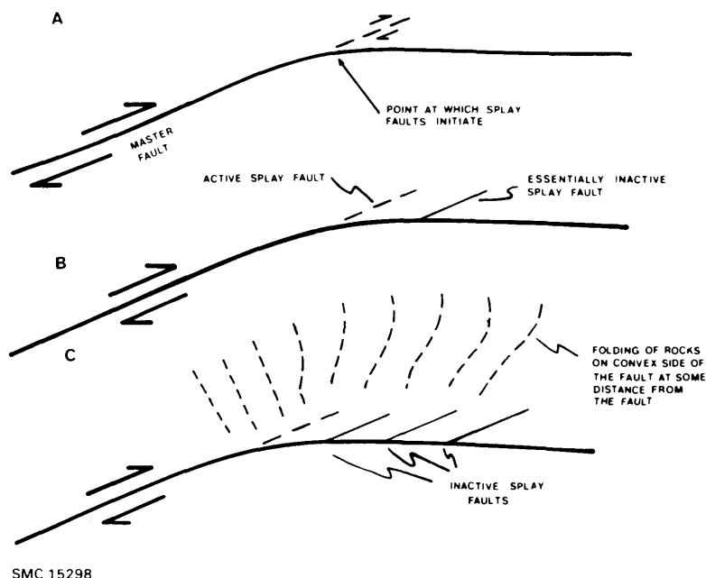
Figure 10. Inferred manner of formation of splay faults associated with a bend in the master fault.
