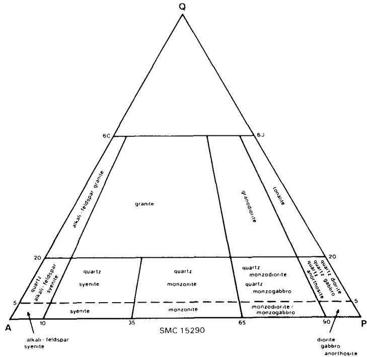
Figure 3. Classification system used for plutonic rocks in the Calm Lake area (after Streckeisen 1976).
