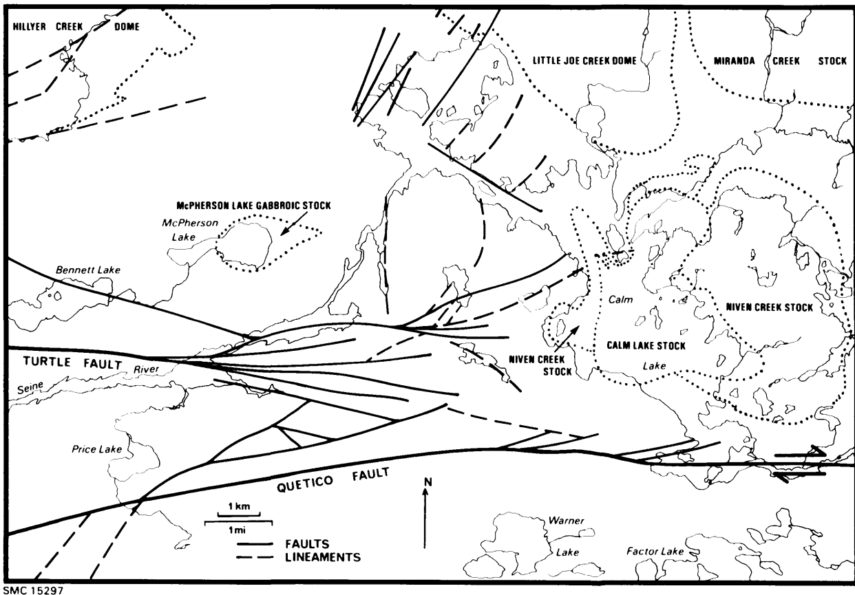
Figure 9. Fault and lineament pattern in the Calm Lake area.
