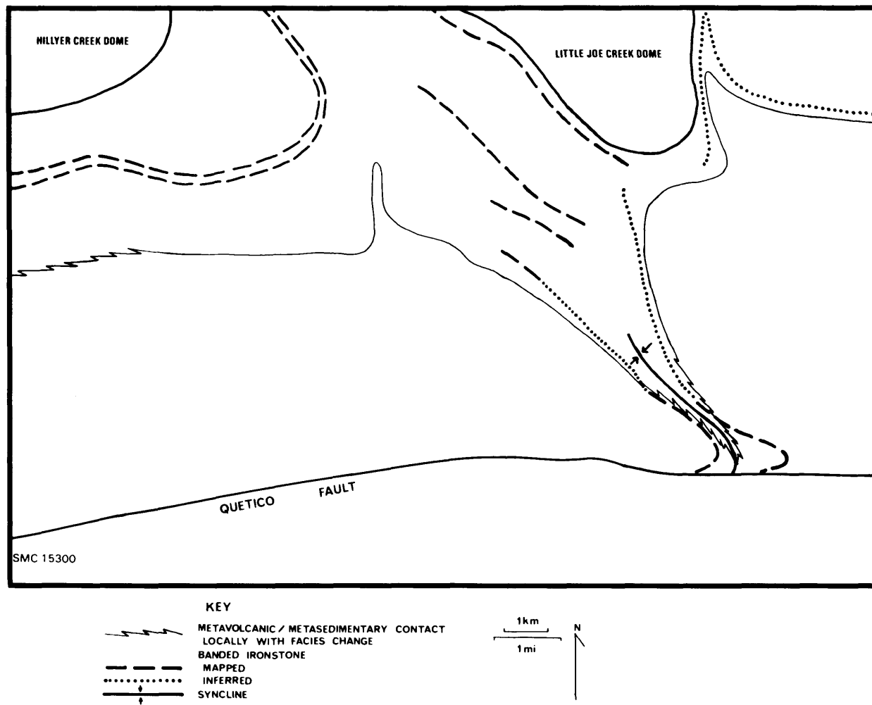
Figure 12. Speculative form of the sedimentary-volcanic contact prior to the emplacement of the Calm Lake and Niven Creek Stocks.
