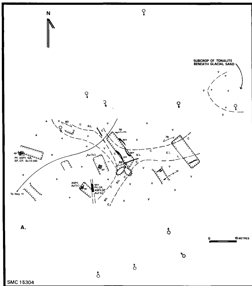
Figure 16a. Geological sketch map of the Mayflower prospect. Modified from Wilkinson (1980).
