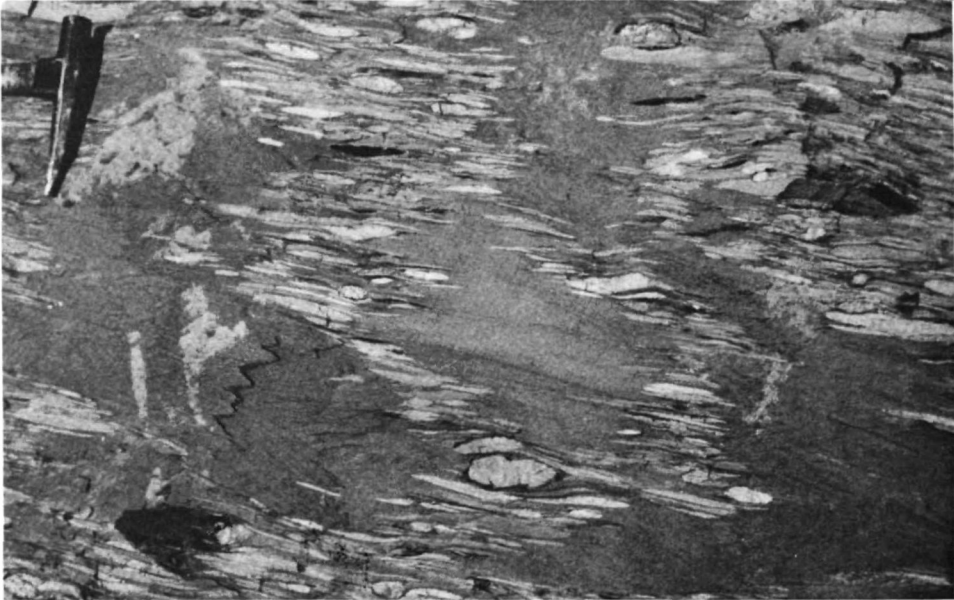
Photo 3. Thin coalescing conglomerate beds in arenite. The tectonic foliation and direction in which individual clasts have been elongated is perpendicular to the bedding. Location: road cut on Highway 11 east of Price Lake.
