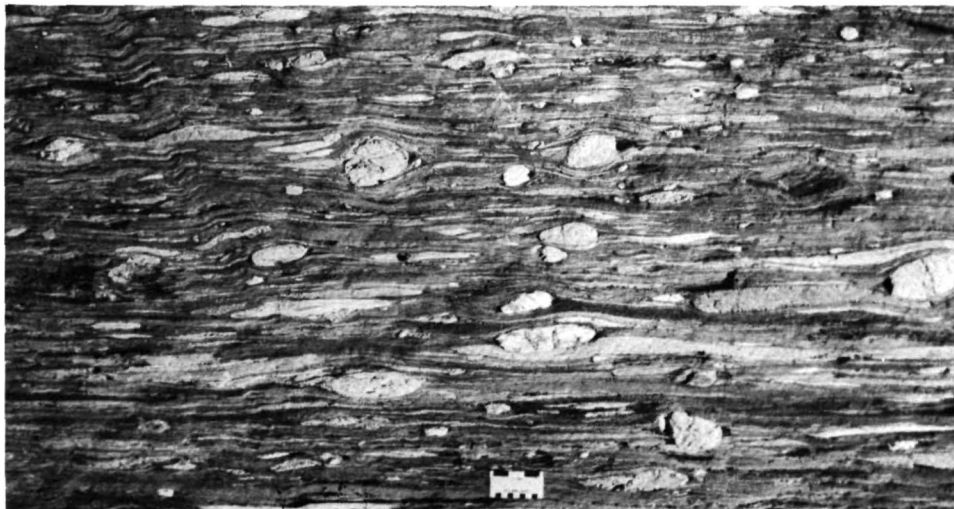
Photo 4. Typical appearance of the Seine conglomerate. Granitoid, felsic metavolcanic, and chert clasts have a high sphericity (1:1 to 1.5:1 length to width). Dioritic and intermediate metavolcanic clasts are elongated (2:1 to 20:1). In contrast, mafic metavolcanic clasts are extremely highly elongated and difficult to recognize ( \gg 20:1). Location: Sturgeon Falls dam.
