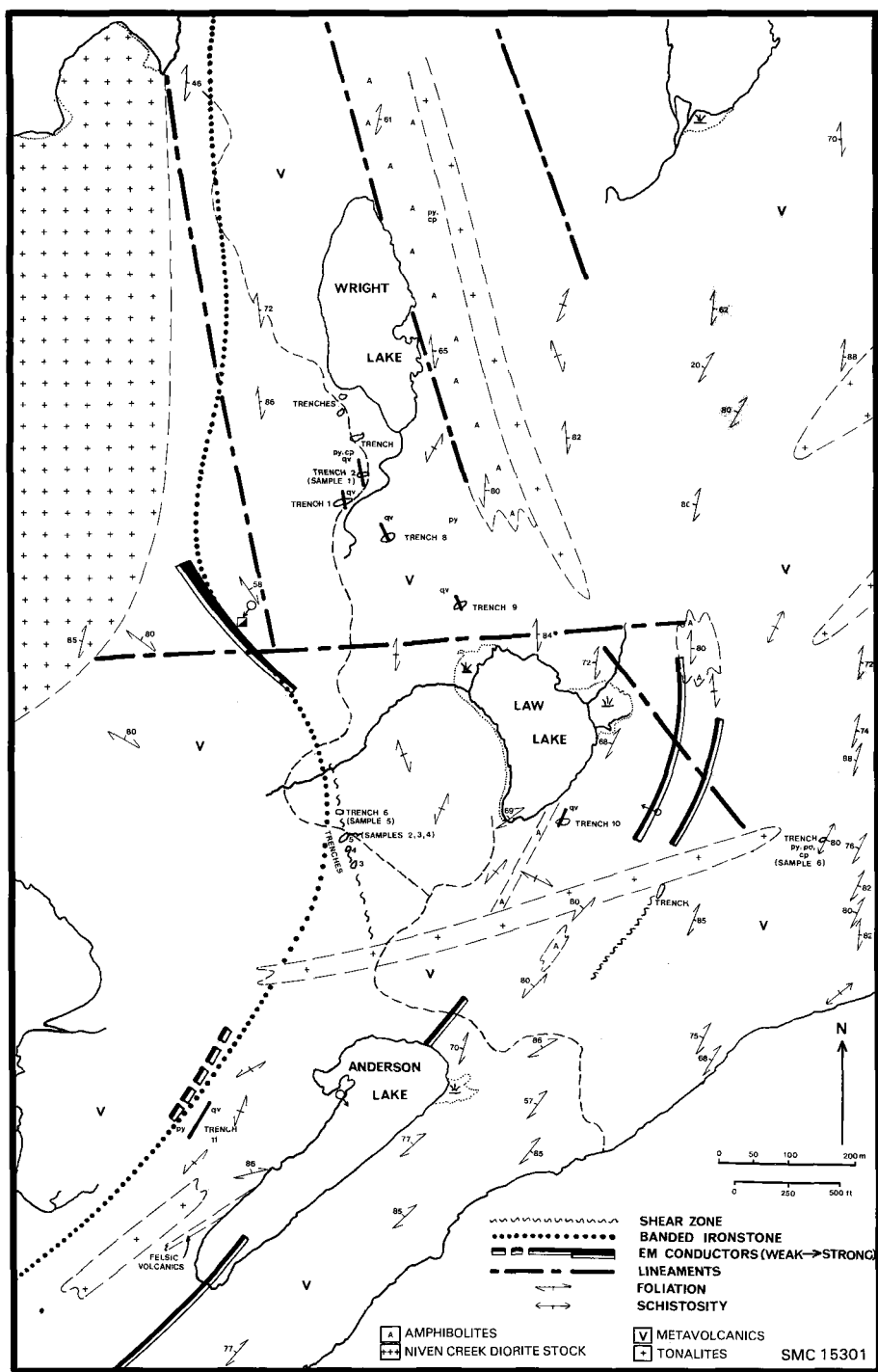
Figure 13. Geological sketch map of the Law occurrence. Geology by S.L. Fumerton, 1979 and 1980, supplemented by information from Hawley (1930) and Regional Geologist files, Ontario Ministry of Natural Resources, Thunder Bay.
