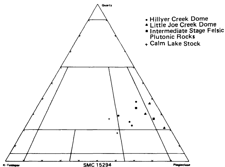
Figure 6. Point counted modal composition of selected plutonic rocks from the Calm Lake area. Names for fields are given in Figure 3.
