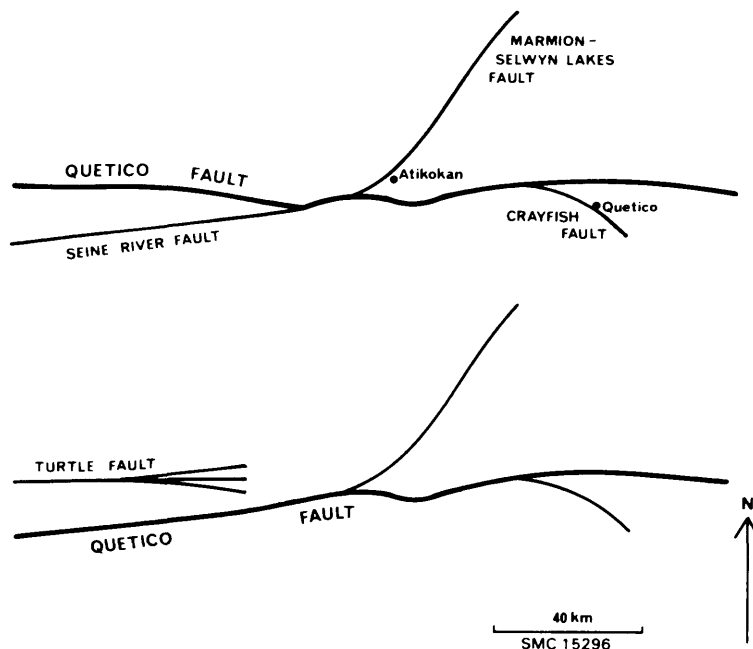
Figure 8. Names and correlation of major faults in the vicinity of the map-area as suggested by previous workers (top diagram) (Schwerdtner et al. 1979; Wood 1980), and by the author (bottom diagram).
