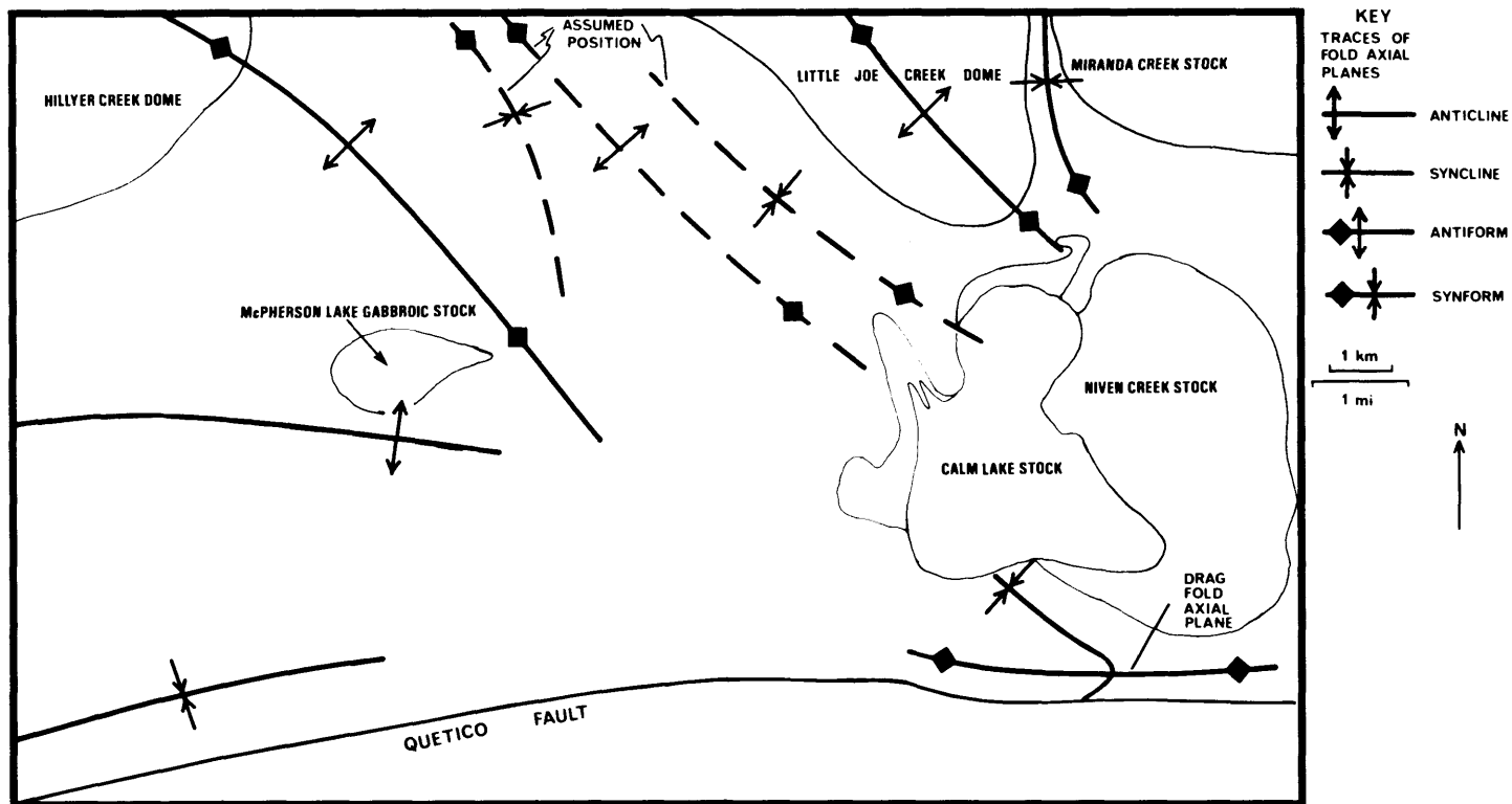
Figure 11. Position of axial planes to anticlines, synclines, antiforms and synforms within the part of the Wabigoon Subprovince in the Calm Lake area.
