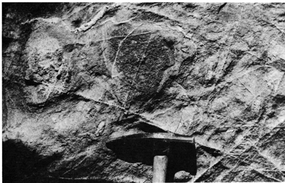
Photo 6. Calm Lake conglomerate containing network of alteration along narrow veins. Location: southeast shore of Hepburn Bay.
