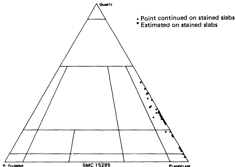
Figure 7. Modal compositions of the felsic to intermediate intrusive rocks, diorite-tonalite stocks, from the Calm Lake Area. Names for fields are given in Figure 3.
