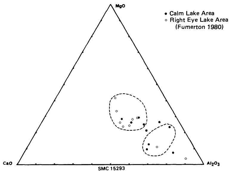
Figure 5. CaO-MgO-Al 2 O 3 plot for metavolcanics from the Calm Lake and Right Eye Lake (Fumerton 1980) areas. Fields enclose all the tholeiitic data, illustrating two distinct compositional ranges. Remaining data points are from the calc-alkaline pyroclastic rocks.
