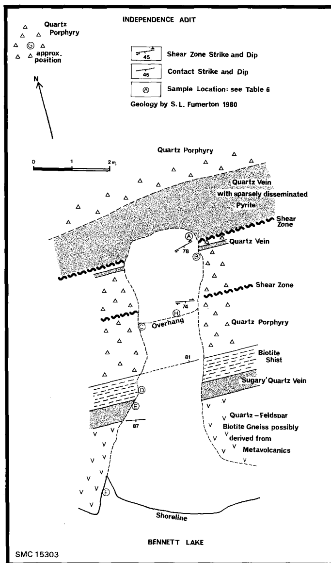
Figure 15. Sketch map of the secondary adit at the former Independence mine property, north shore of Bennett Lake. Geology by S.L. Fumerton.
